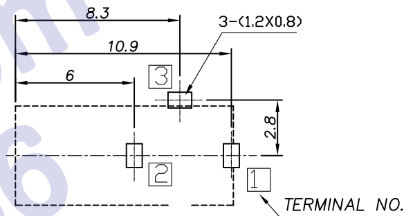
P.C.B Layout (Printed-sided view)
