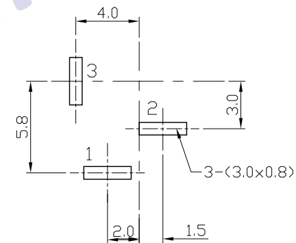
P.C.B LAYOUT VIEW
