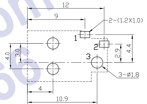
P.C.B LAYOUT VIEW
