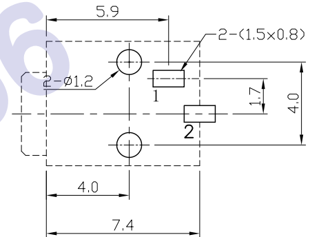
P.C.B LAYOUT VIEW
