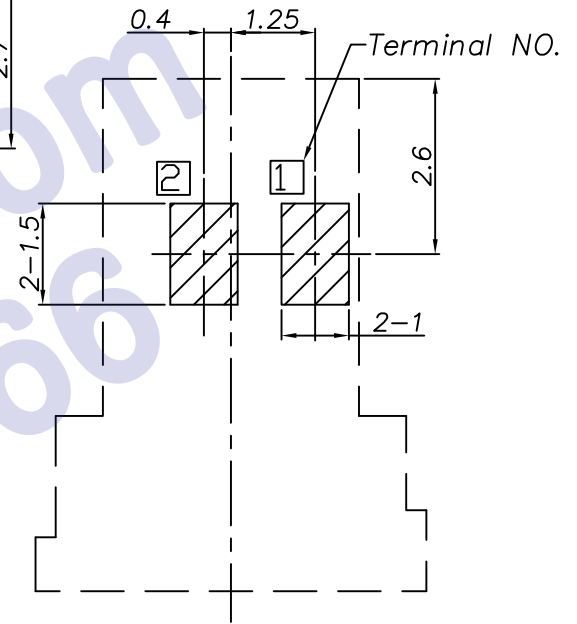
P.C.B Layout (Printed-sided view)
