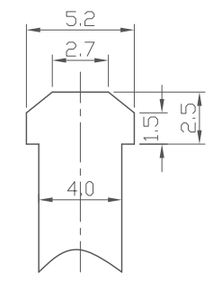
REFERENCED DIMENSION
