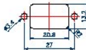
PANEL LAYOUT
