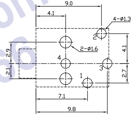
P.C.B LAYOUT VIEW
