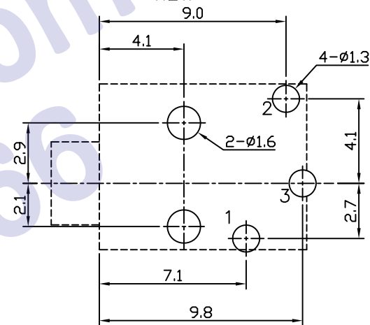
P.C.B LAYOUT VIEW
