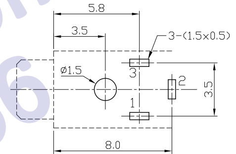
P.C.B LAYOUT VIEW
