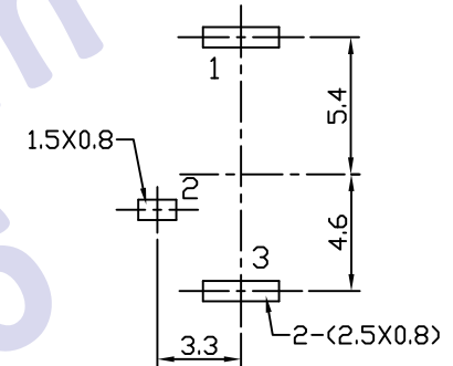
P.C.B LAYOUT VIEW
