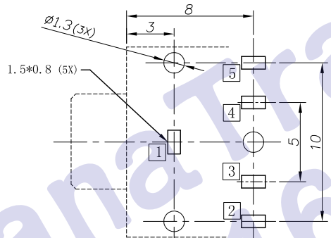
RECOMMENDED P. C. B. LAYOUT UNSPECIFIED TOLERANCE: ±0.05 (BOTTOM VIEW)
