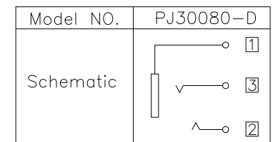
Circuit Diagram Terminal No.
