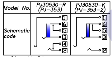
Circuit Diagram □: Terminal No.
