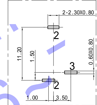
PCB LAYOUT
