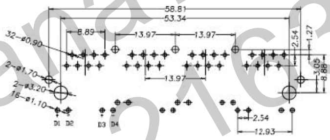
SUGGESTED PCB LAYOUT TOP VIEW
