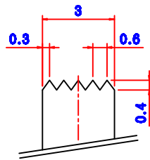
DETAIL KNOB (5/1)
