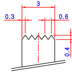
DETAIL KNOB (5/1)
