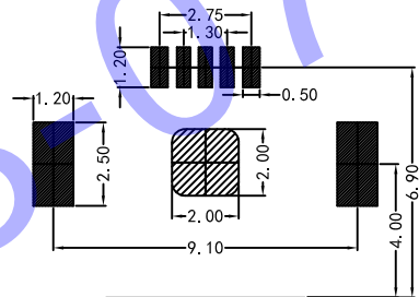
RECOMMENDED PCB LAYOUT PCB图仅供参考
