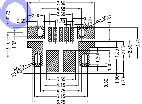
RECOMMENDED PCB PATTERN Tolerance: ±0.05
