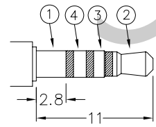
ø2.5 SPECIAL MATE PLUG
