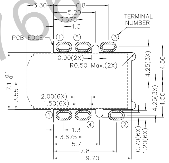
RECOMMENDED SOLDER PAD LAYOUT (TOP VIEW)
